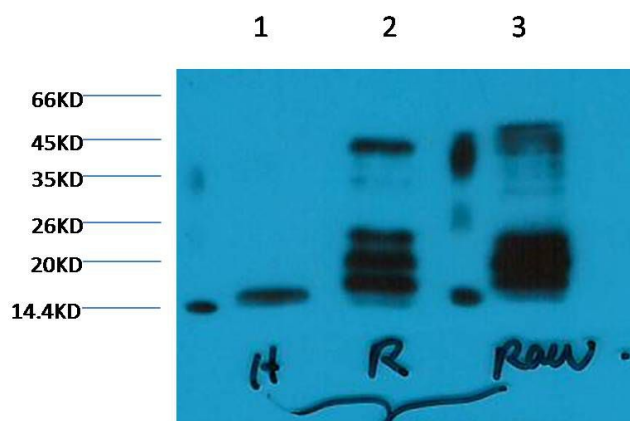
Western blot analysis of 1) Hela, 2) Rat Testis tissue, 3) Raw264.7 with Histone H3 (di methyl K27) Mouse MAb diluted at 1:2000.
